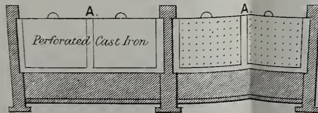
TRANSVERSE SECTION ON LINE A. B.
